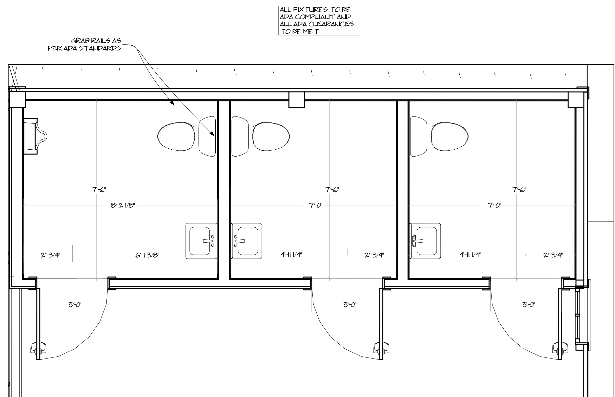
BATHROOM PLAN SCALE 1/2" = 1'-0" *
